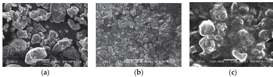
Figure 2. Scanning Electron Microscopic analysis. (a) Curcumin 500×; (b) curcumin nanoparticles 5000×; (c) curcumin nanoparticles 20,000×.
