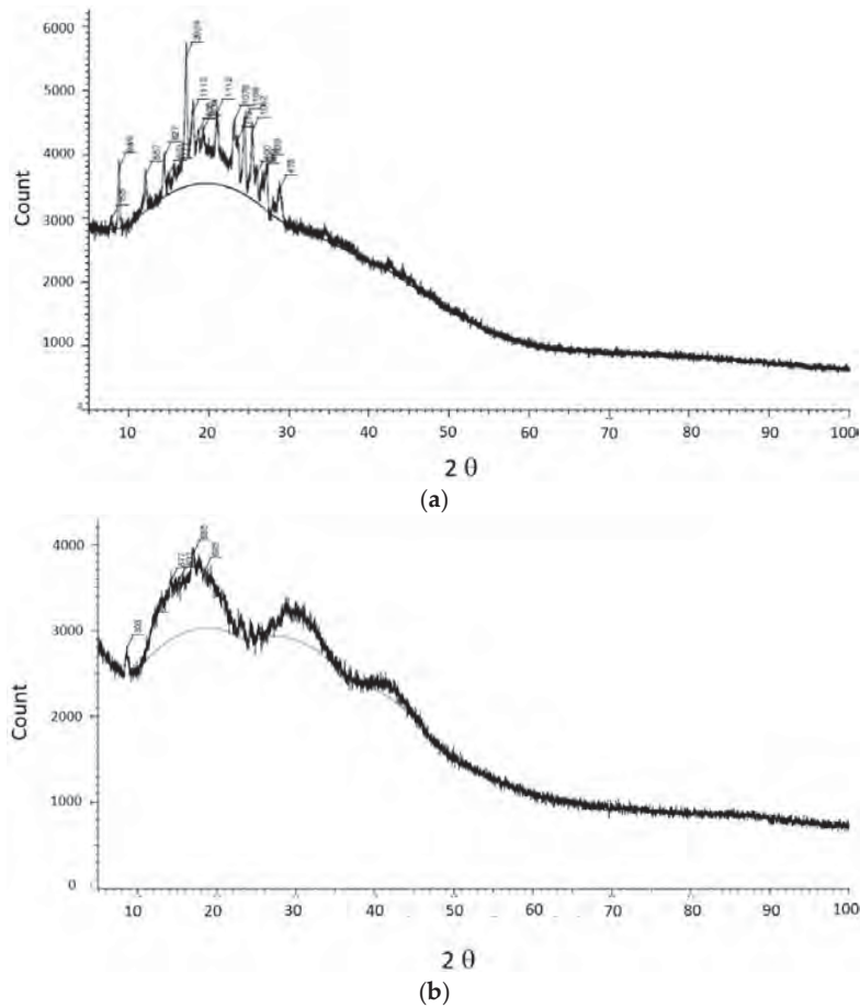
Figure 4. The X-ray diffractograms of curcumin (a) and curcumin nanoparticles (b).
