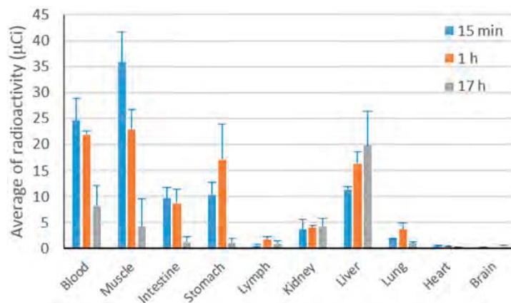
Figure 7. The accumulation profile of ^{131} I-labeled curcumin after intravenous administration to male healthy Webster mice.
