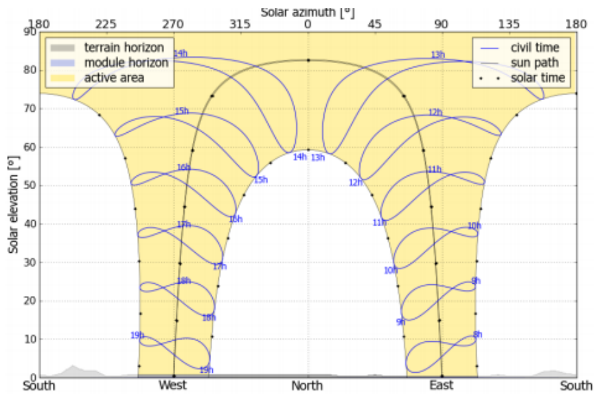
Fig. 6. Sun Path over a year in Surabaya
