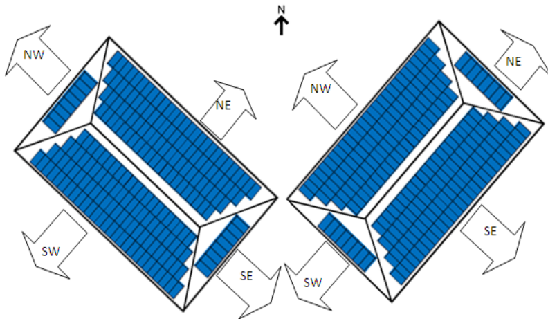
Fig. 4. Theoretical sitting of PV panels for different building orientation
