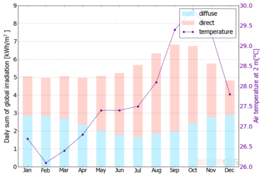
Fig. 8. Global irradiation and air temperature in Surabaya
