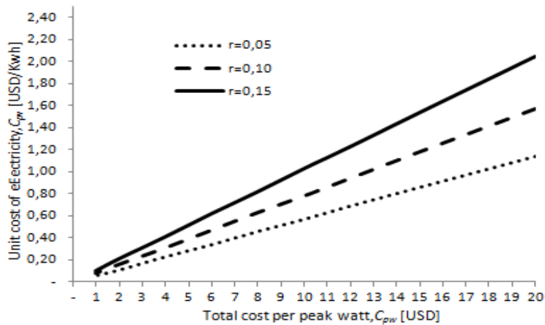
Fig. 10. The unit cost of PV electricity versus total cost per watt with various of rate of return, r
