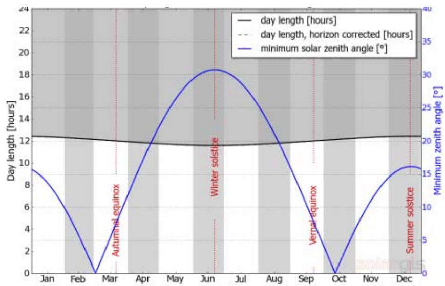
Fig. 6. Sun Path over a year in Surabaya
