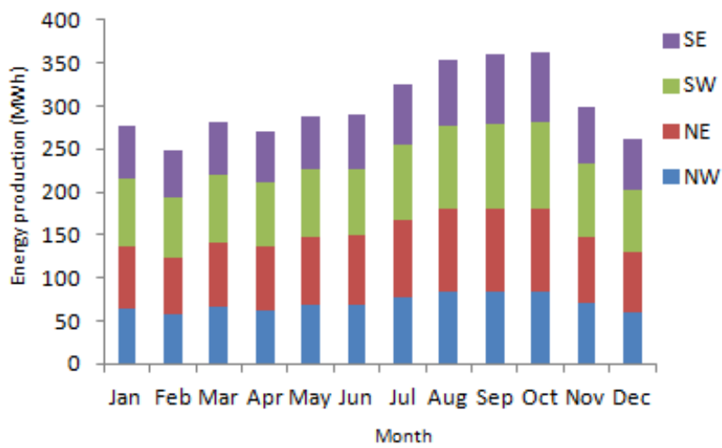
Fig. 9. Monthly energy production of rooftops mounted PV system
