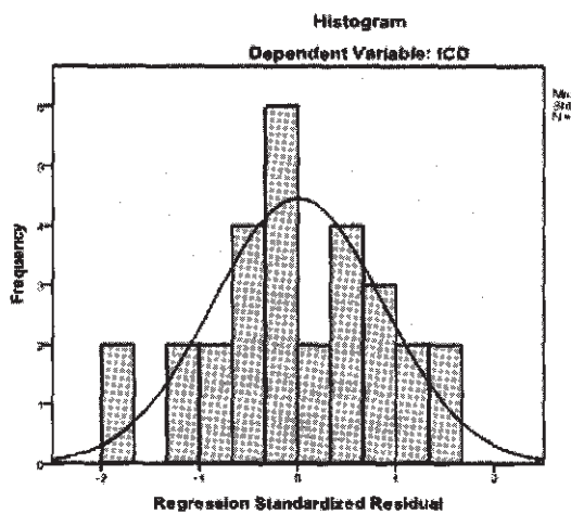
Gambar 1 Histogram Normal Probability Plot
