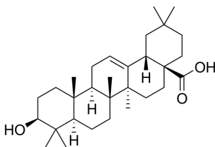
Figure 1. The chemical structure of oleanolic acid
