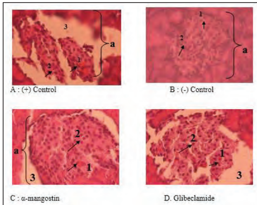
Fig. 3. Islet of Langherans (40 × 10 magnification).
