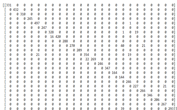
Gambar 7. Confusion Matrix CNN-2 + Gaussian LPF
