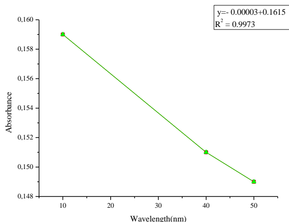
Figure 3. Linear curve analysis of mercury using a solution of Ni(OH) 2 nanoparticles at a volume of 5 mL
