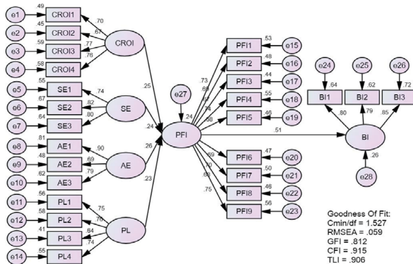
Gambar 2 Model Struktural
