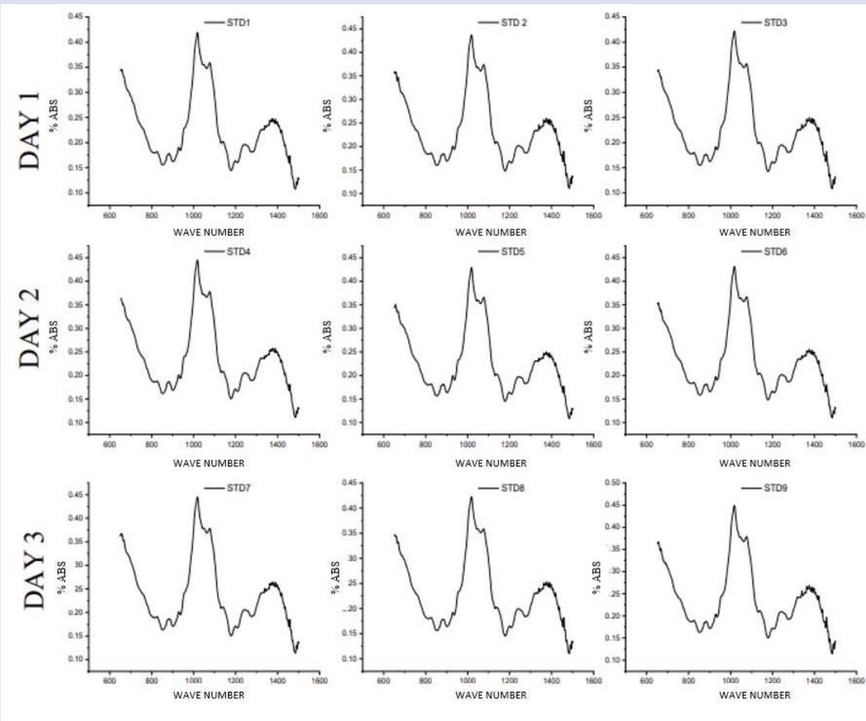
Figure 6: Absorbance spectrum (Finger Print) - standard replication in 3 days.
