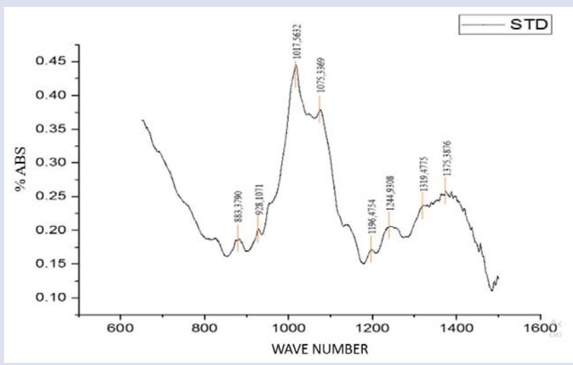
Figure 8: Absorbance spectrum standard.
