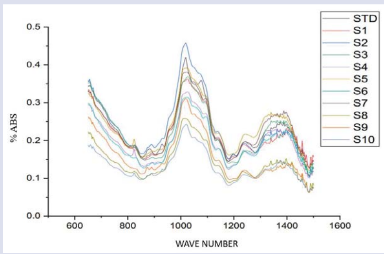
Figure 9: Absorbance spectrum standard and 10 sample overlay.
