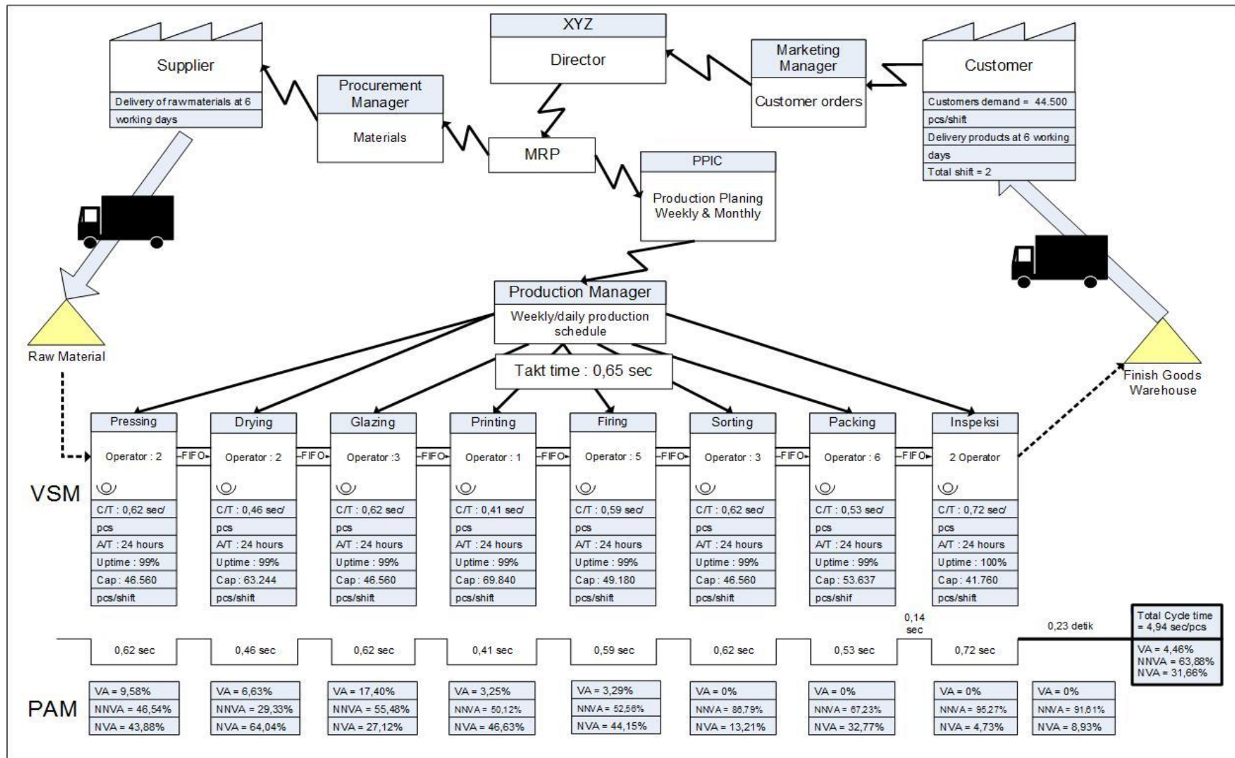
FIGURE 8. Proposed state map Analysis
