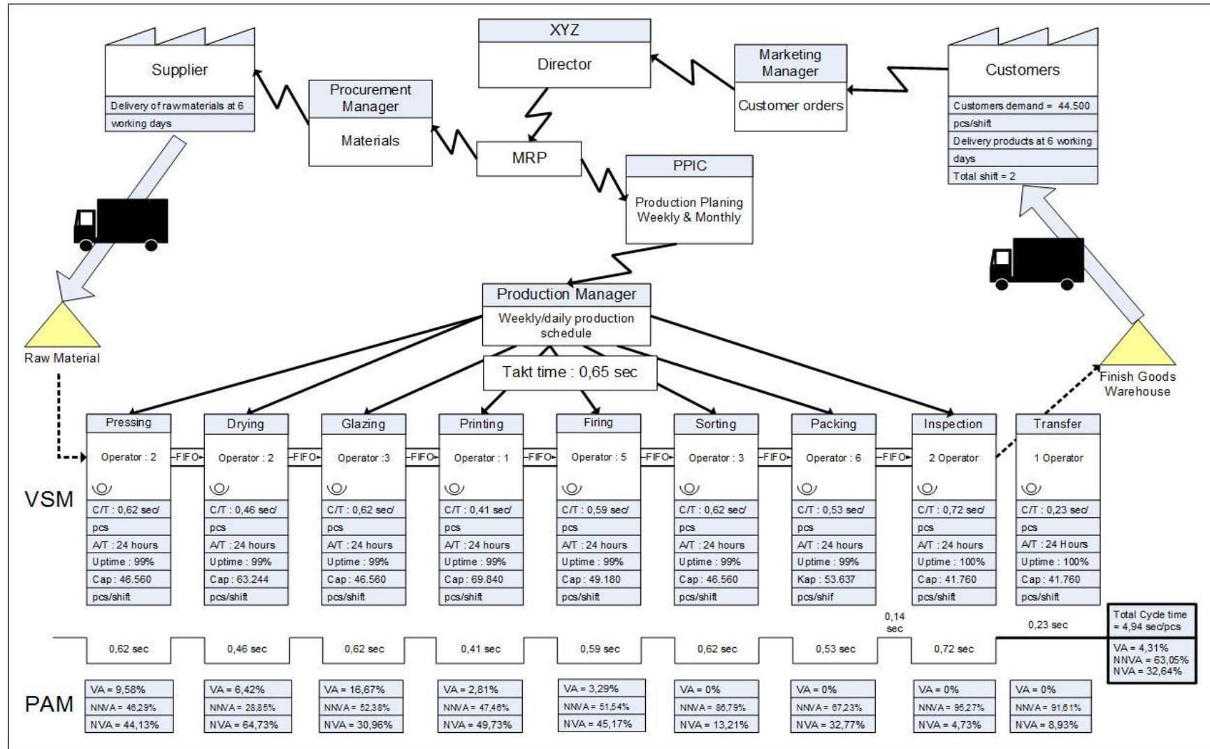
Gambar 3. Current state map
