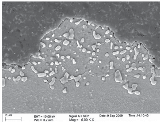
Fig. 2: Scanning electron micrograph of interface layer of sialon and 7.5%-Cr steel joint
