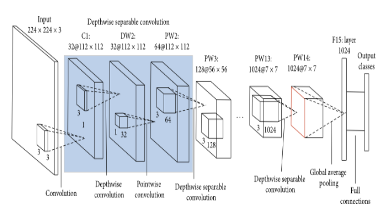
Fig. 4. MobileNetV2 architecture
