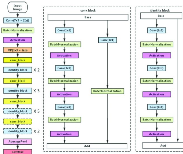
Fig. 1. ResNet50 architecture
