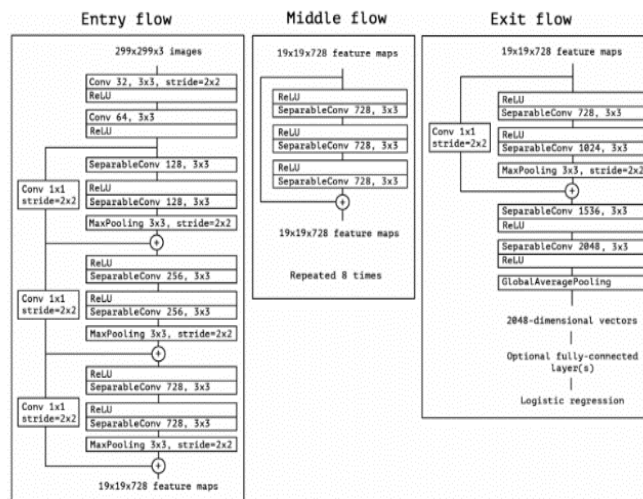
Fig. 6. Xception architecture
