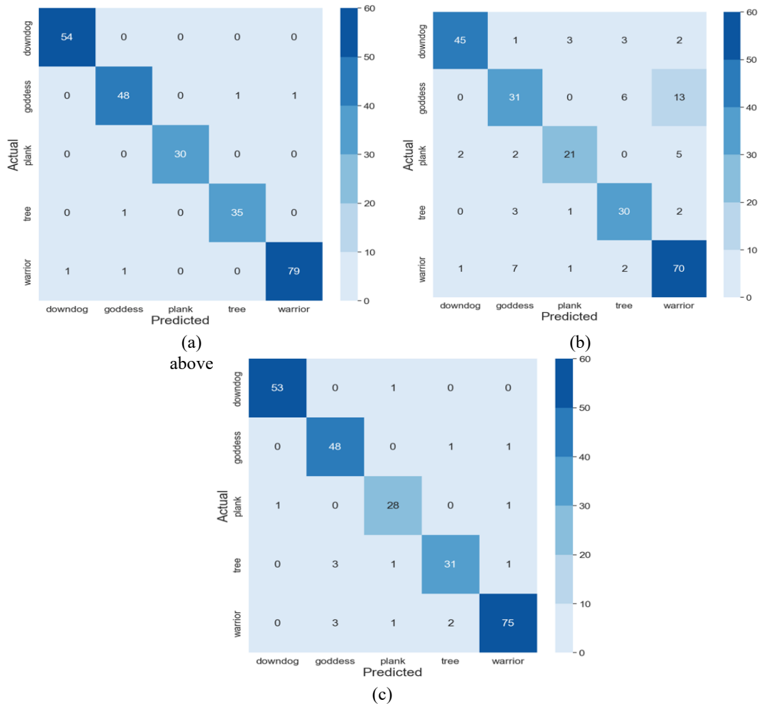
Fig. 9. Confusion matrix of MobileNektV2 (a), Xception (b), dan ResNet50 (c)
