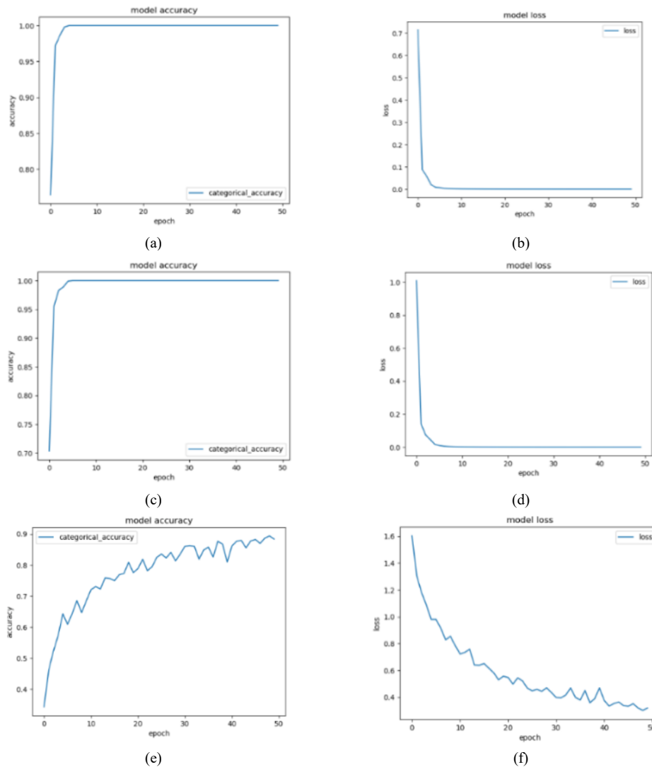
Fig. 8. Accuracy and loss graph of MobileNetV2 (a)(b), Xception (c)(d), and ResNet50 (e)(f)
