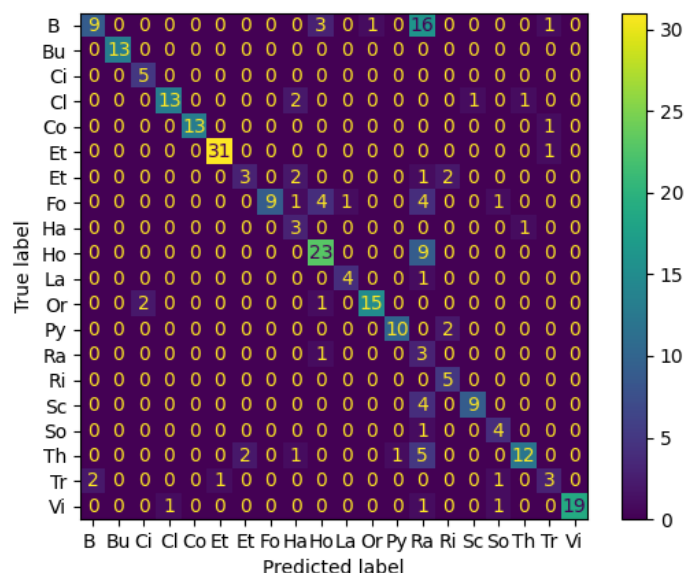
Gambar 18. Confussion Matrix GoogleNet
