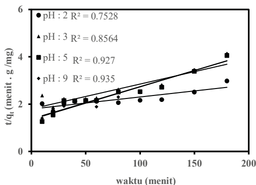
Gambar 3. Plot Model Kinetika Pseudo Second Order
