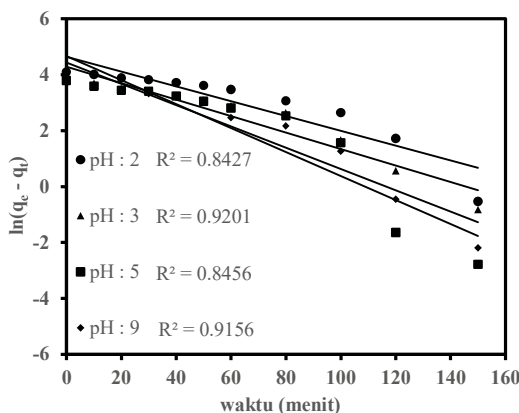
Gambar 2. Plot Model Kinetika Pseudo First Order
