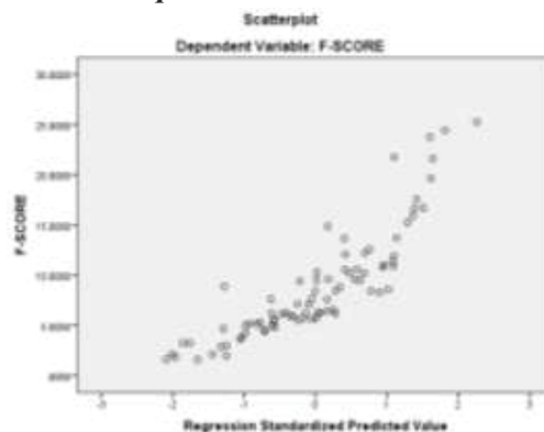
Gambar 4.2 Scatterplot Heteroskedastisitas
