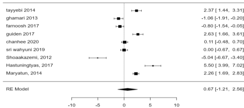
Gambar 2. Forest Plot
