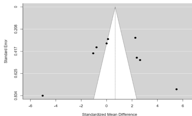
Gambar 3. Funnel Plot
