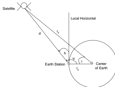
Gambar 2. Geometri Kalkulasi Sudut Elevasi (Pratt T., C.W. Bostian. 1986. Satellite Communication . New York : John Wiley & Sons.)
