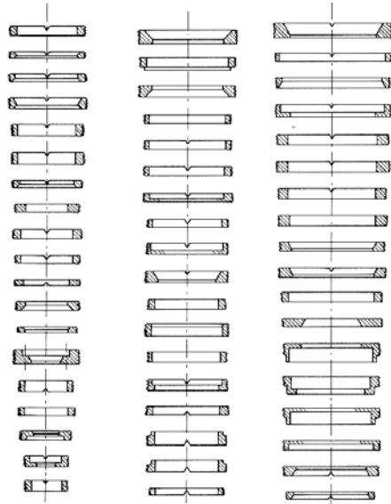
Gambar 1. A Design Family [source: Chang, Wang and Wysk, CAM, pub.: prentice-hall]
