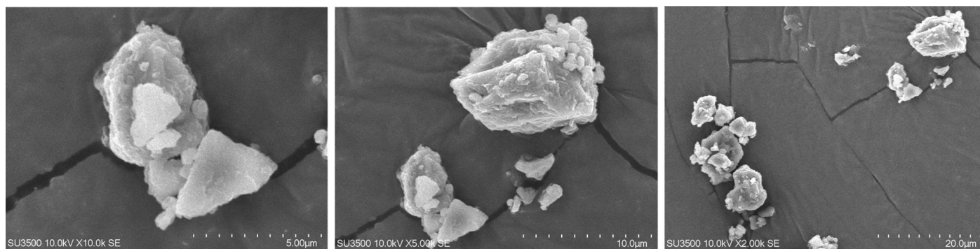
Figure 3. SEM Analysis of MPN Morphology
