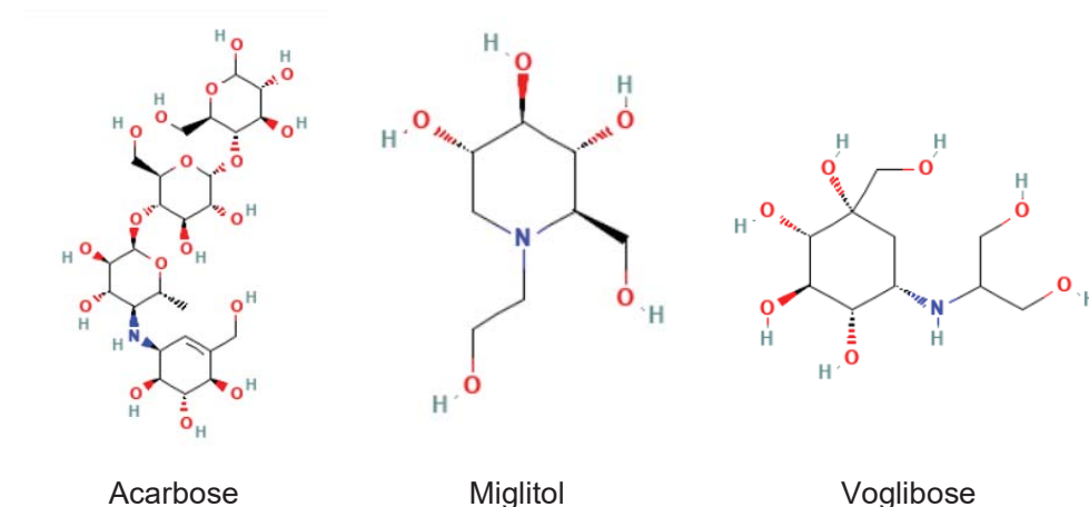
Figure 1. Structure of Acarbose, Miglitol, and Voglibose ( PubChem )
