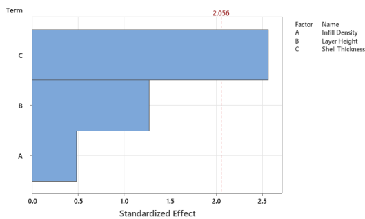
Figure 4. Pareto Chart of Flexural Strength-and-Mass Ratio
