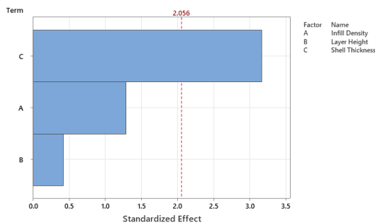
Figure 5. Pareto Chart of Flexural Modulus
