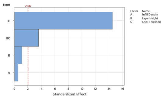
Figure 6. Pareto Chart of Strain
