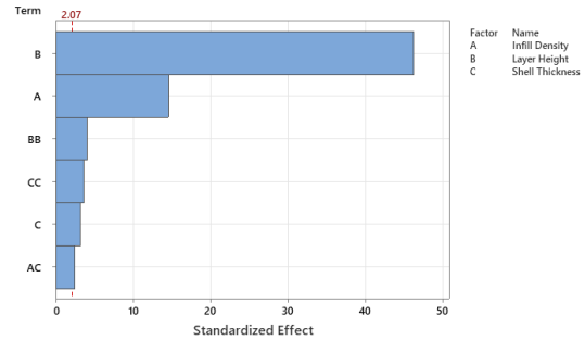
Figure 7. Pareto Chart of Printing Time
