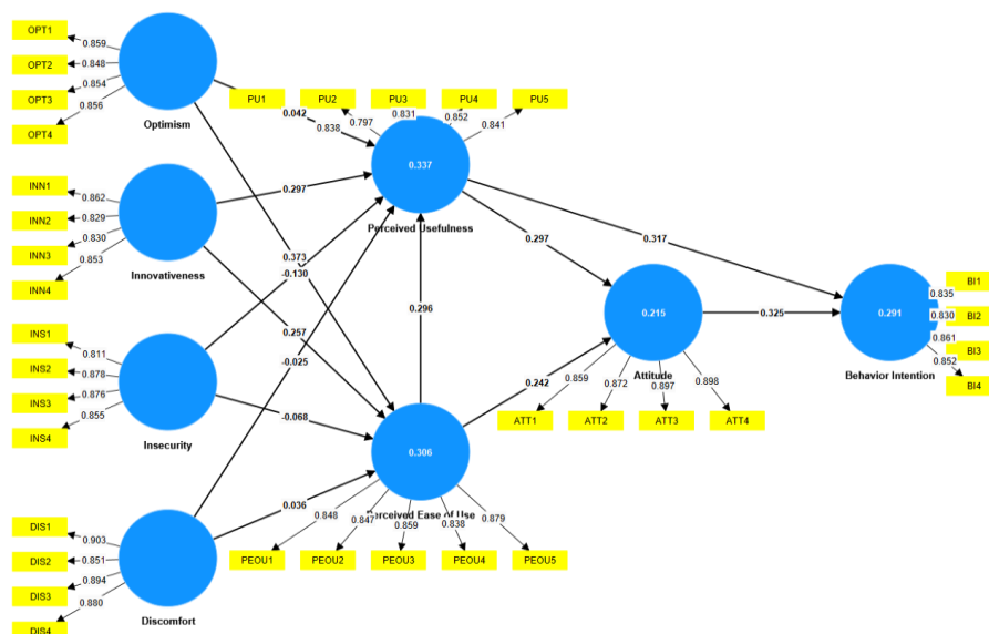
Figure 1. SmartPLS 4 Output
