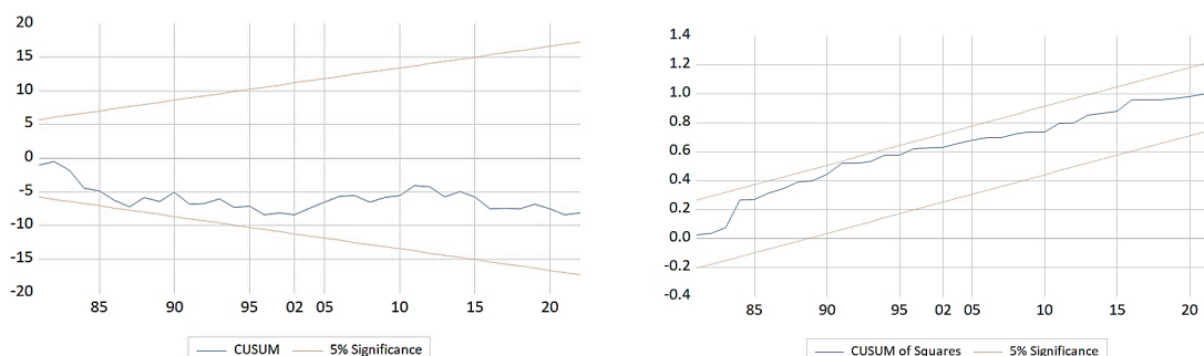
Figure 2. CUSUM and CUSUM of Squares
